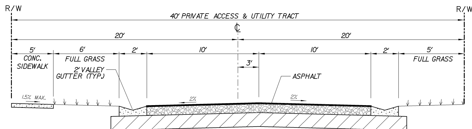
TYPICAL ROAD SECTION 40' PRIVATE ROAD TRACT N.T.S.
