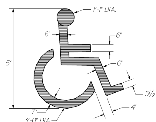
HANDICAP SYMBOL PAINT DETAIL N.T.S.
