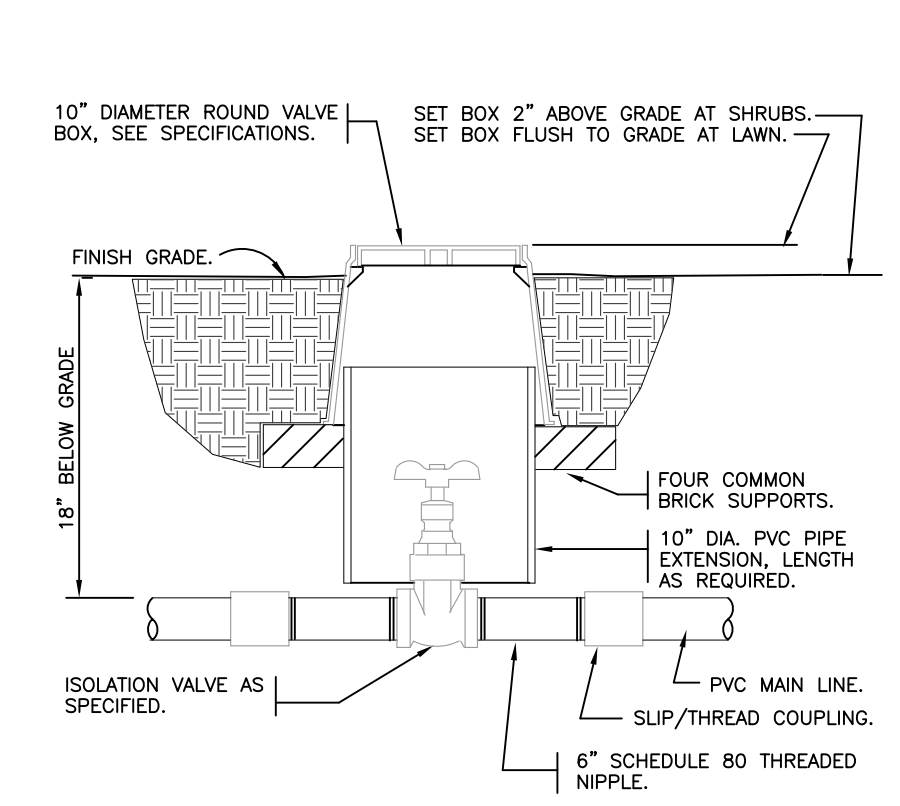
9 BRASS ISOLATION VALVE 1 1/2" = 1'-0" 32 8406.33-01
