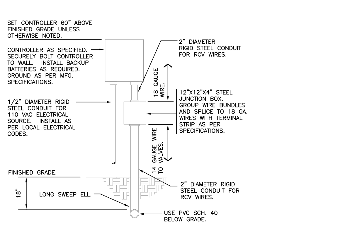
10 WALL MOUNT CONTROLLER 1" = 1'-0" 32 8409.13-02
