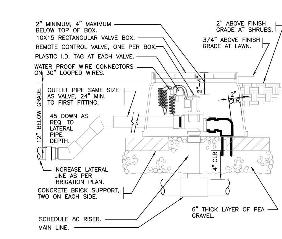
8 ELECTRIC REMOTE CONTROL VALVE 1 1/2" = 1'-0" 32 8406.13-01
