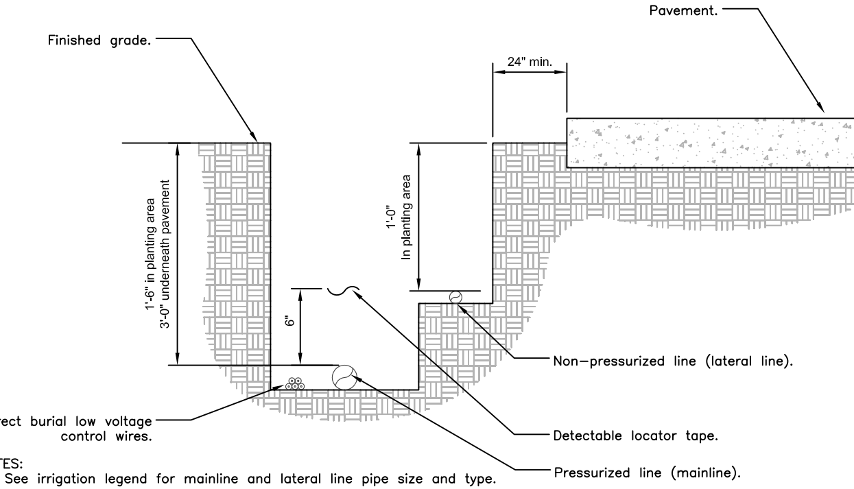
12 IRRIGATION TRENCHING 1 1/2" = 1'-0" FX-IR-FX-AUXEQ-08
