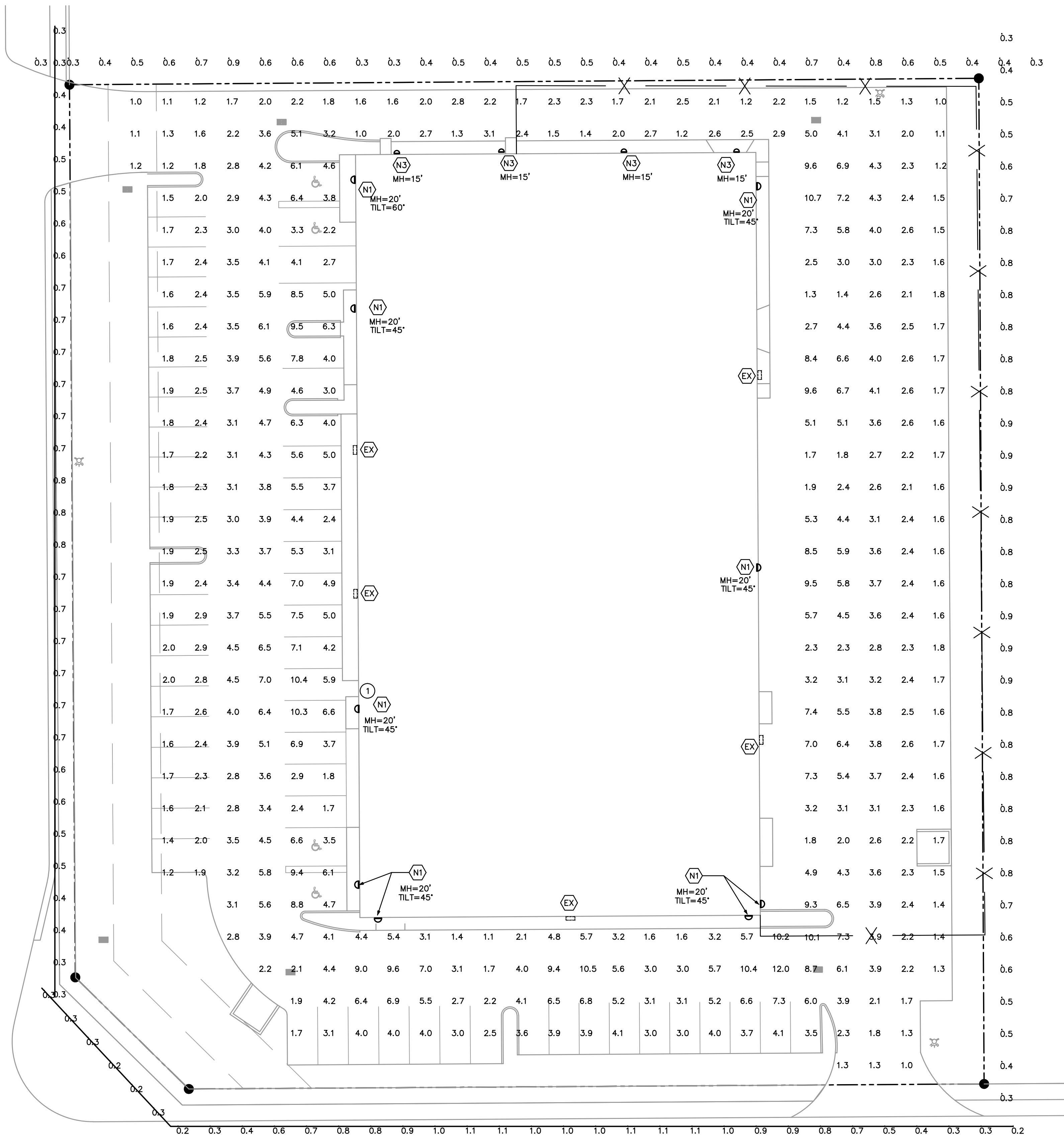
SITE PHOTOMETRIC PLAN 1"=20'-0" NORTH
