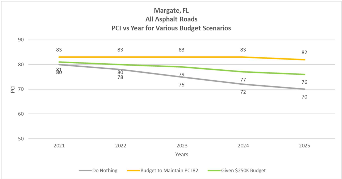
Figure 2-4 – Margate, FL – All Asphalt Roads Scenarios Summary
