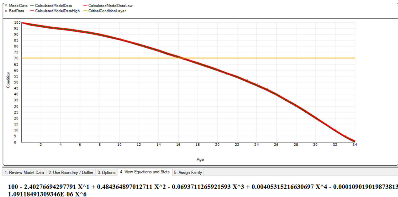
Figure A-1 Margate, FL All Roads - Pavement Performance Curve
