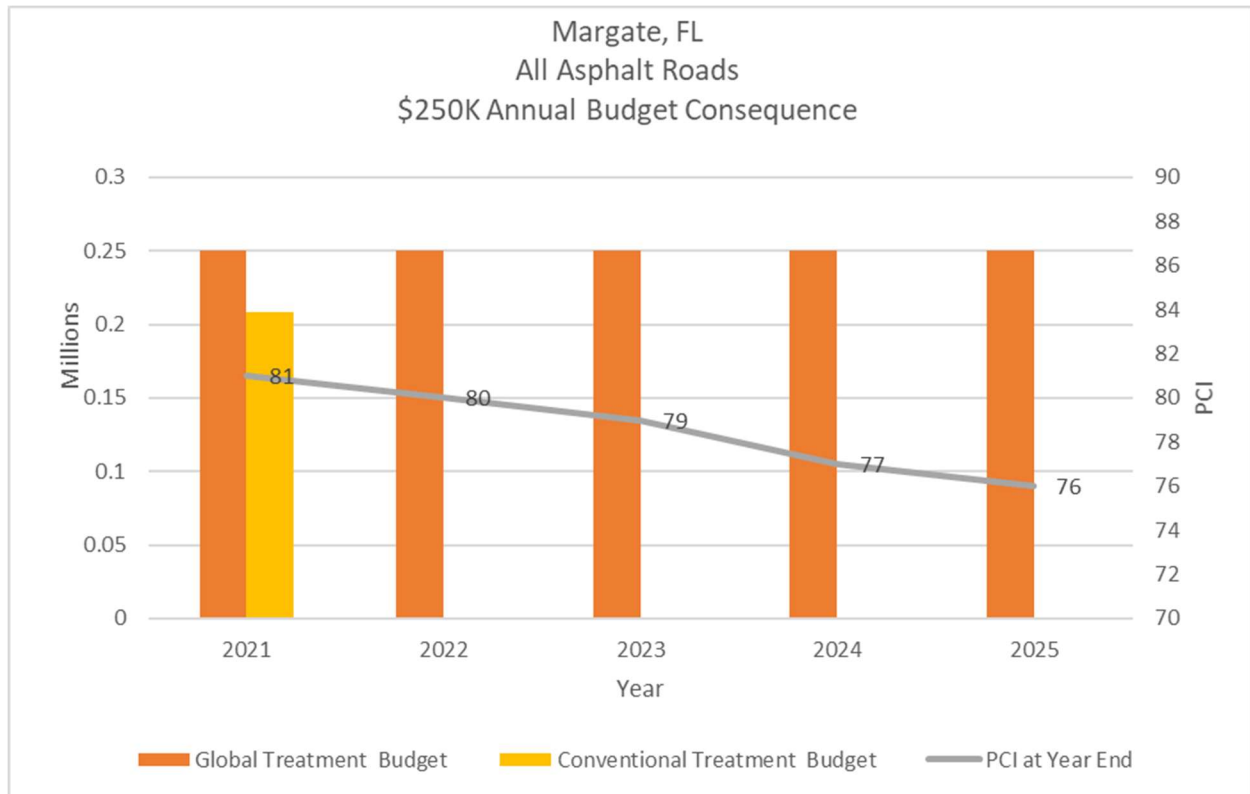
Figure 2-3 – Margate, FL – All Asphalt Roads $250K Given Budget Consequences
