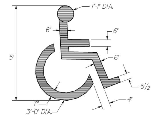
HANDICAP SYMBOL PAINT DETAIL
