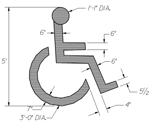
HANDICAP SYMBOL PAINT DETAIL
