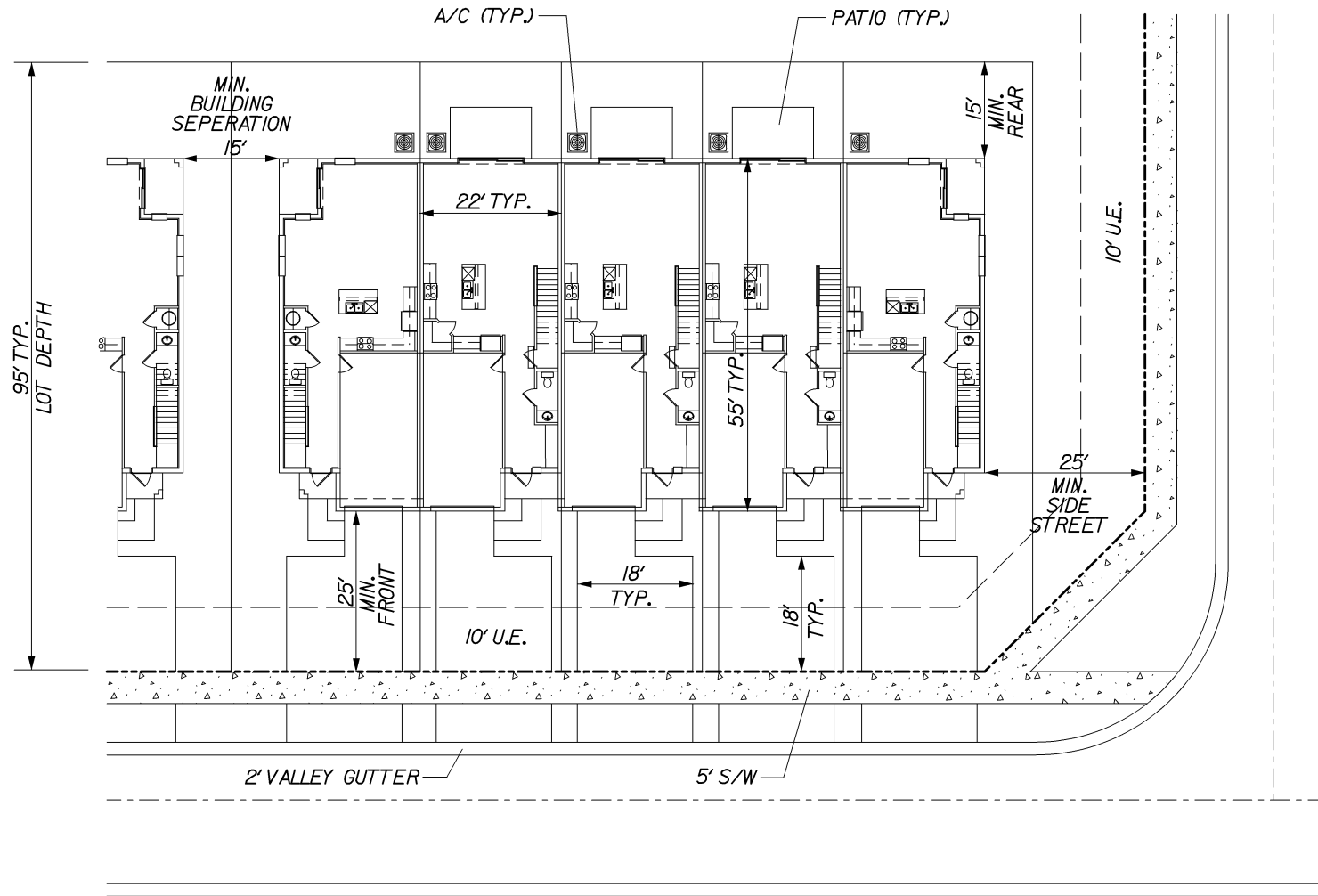
TYPICAL BUILDING DETAIL
