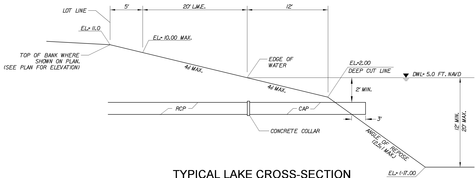
TYPICAL LAKE CROSS-SECTION N.T.S.
