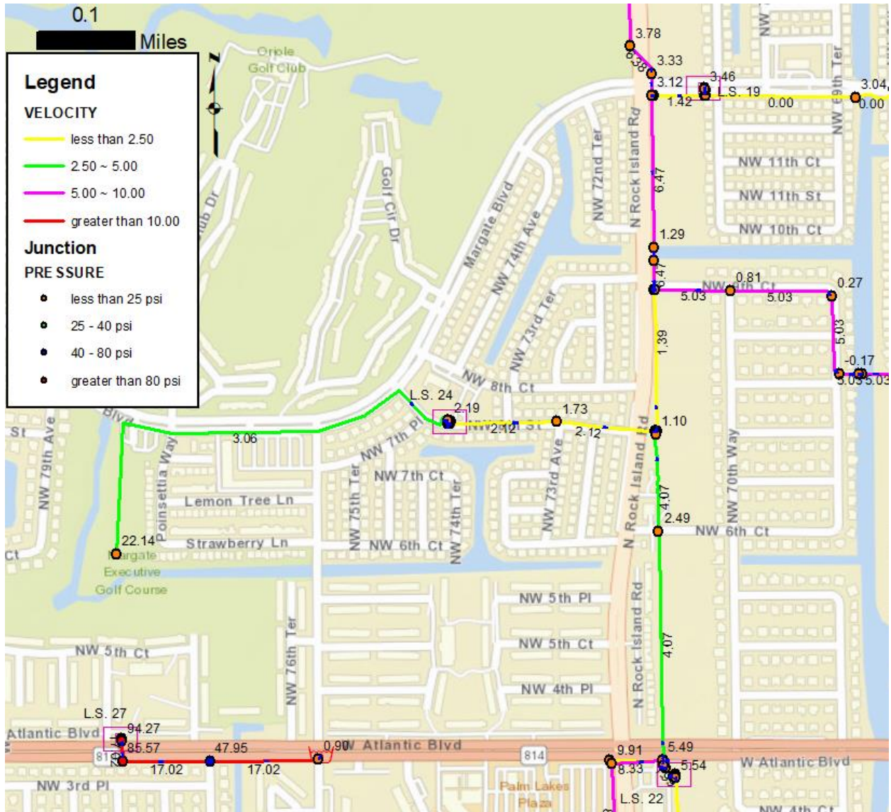
Figure 9 –Wastewater PHF Springdale Townhomes Results
