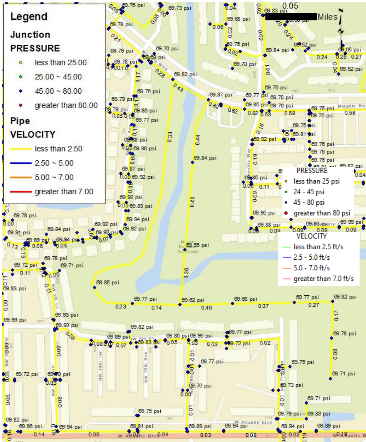
Figure 7 – Potable Water PHF Springdale Townhomes Results
