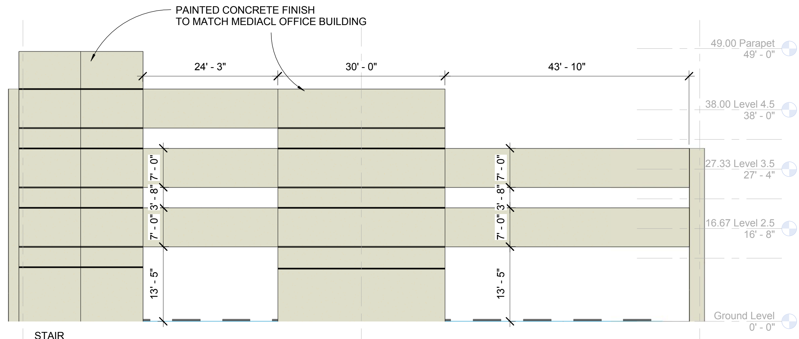
② Elevation West 3/32" = 1'-0"
