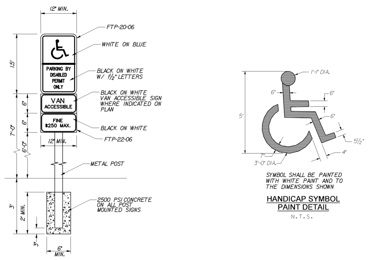
HANDICAP PARKING SIGN N.T.S.
