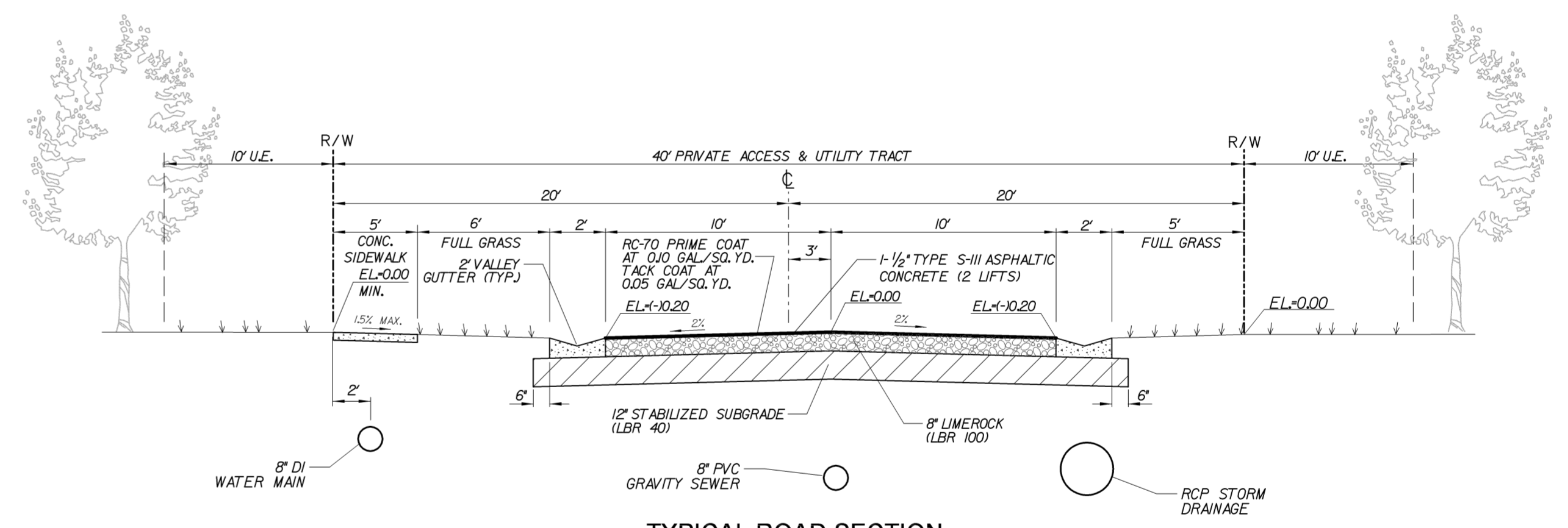
TYPICAL ROAD SECTION 40' ROAD TRACT N.T.S.
