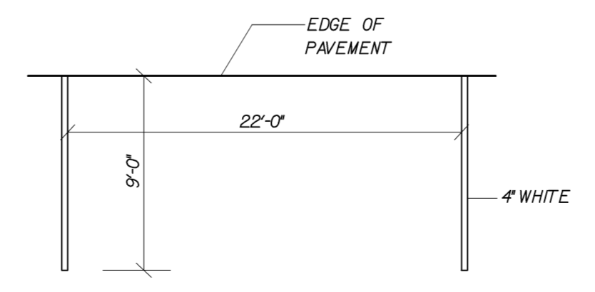
PARALLEL PARKING SPACE N.T.S.
