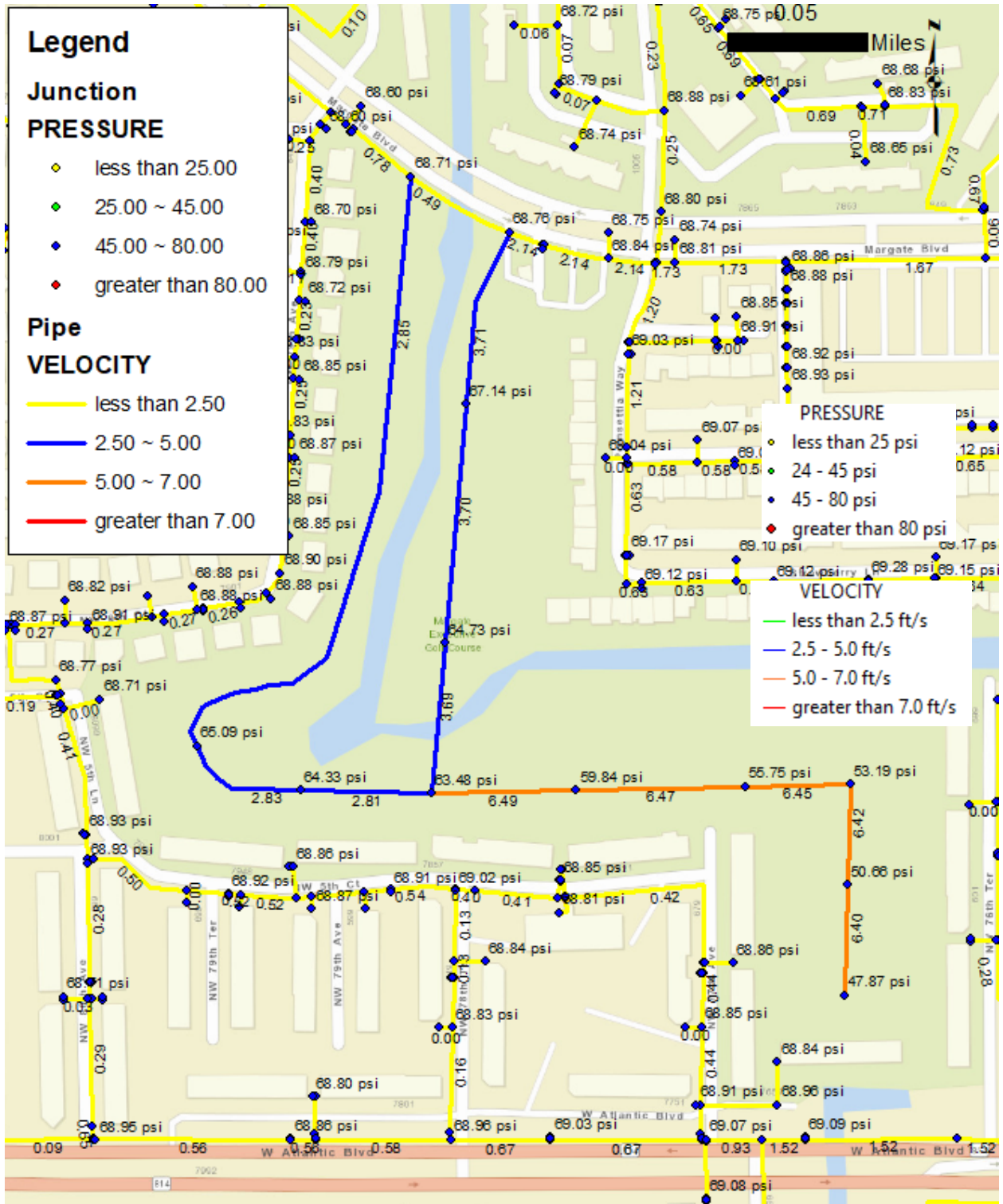
Figure 5 – Potable Water MDD+FF Springdale Townhomes Results
