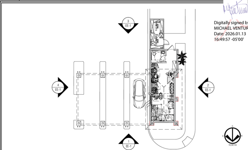
5 KEY PLAN 1/8" = 1'-0"
