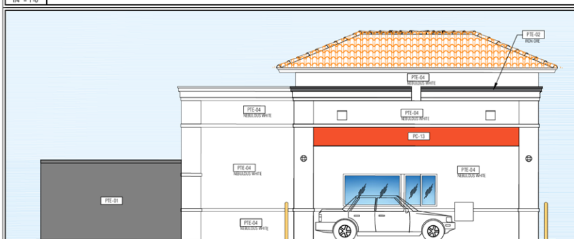
4 PROPOSED EAST ELEVATION 1/4" = 1'-0"
