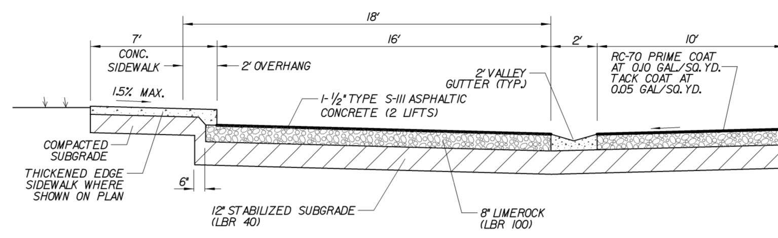
TYPICAL PARKING WITH SIDEWALK DETAIL
