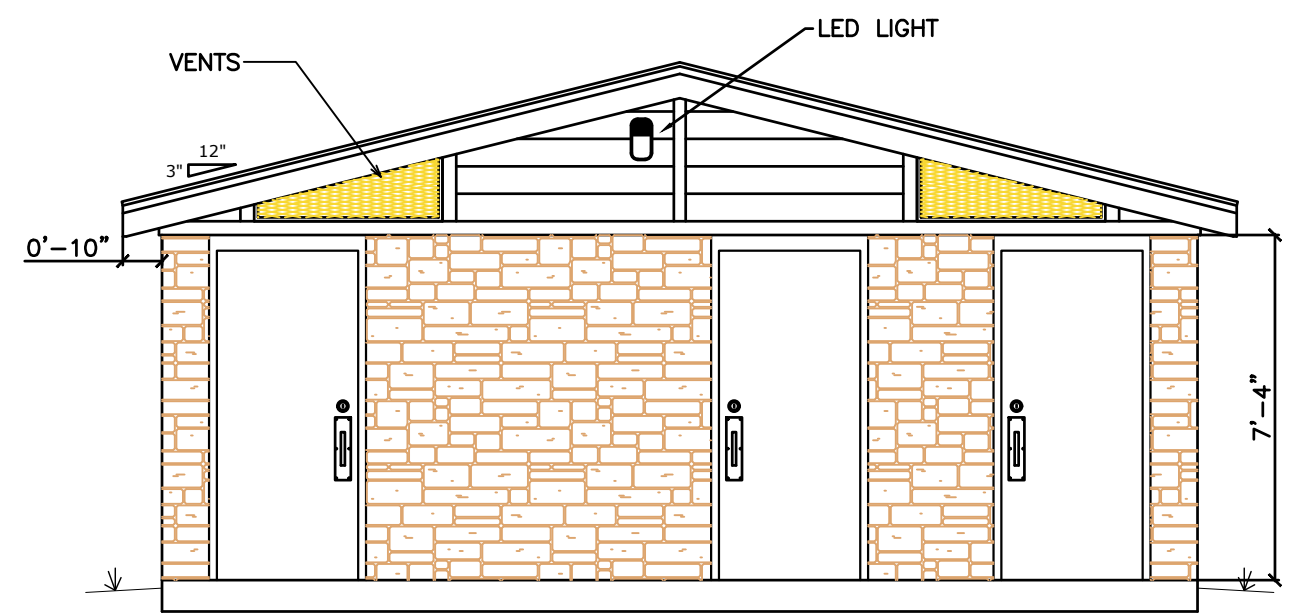
② FRONT ELEVATION
