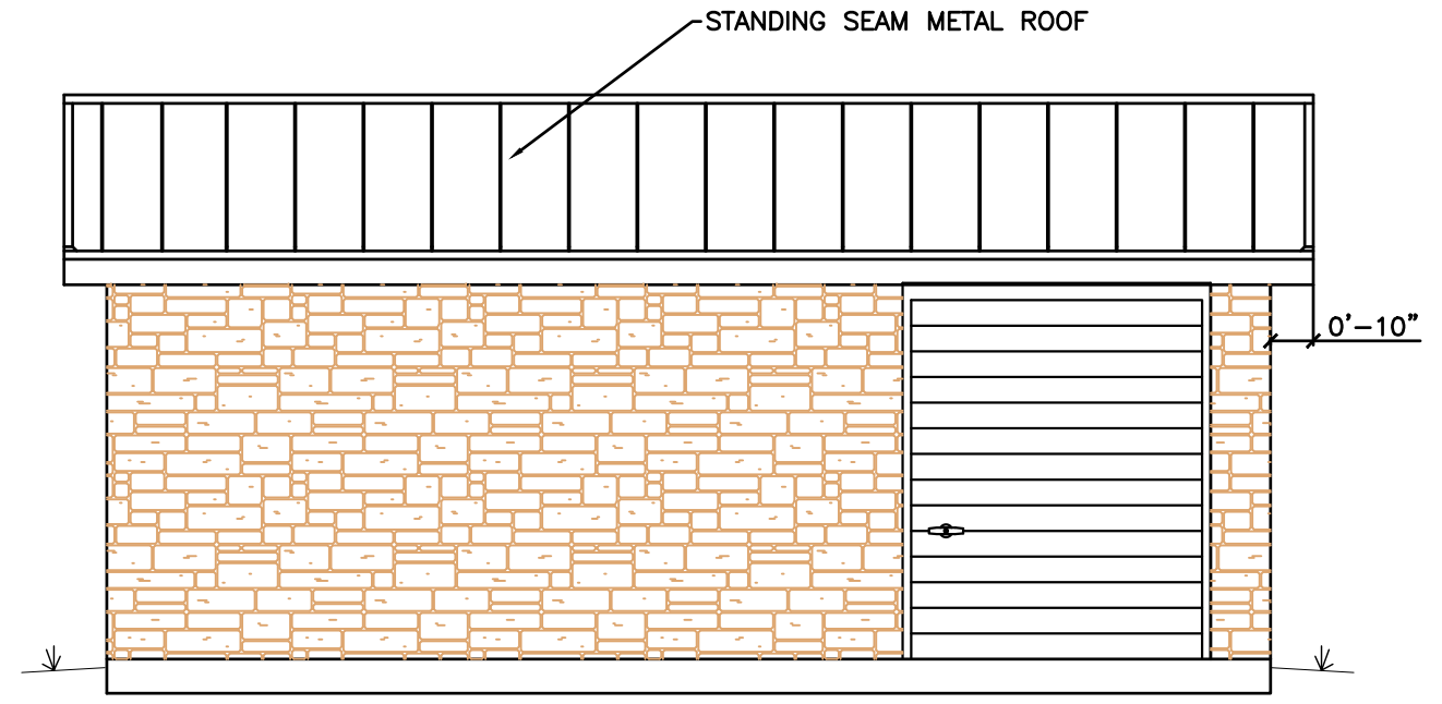
② RIGHT SIDE ELEVATION
