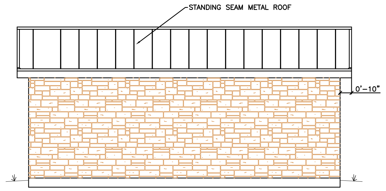
① LEFT SIDE ELEVATION
