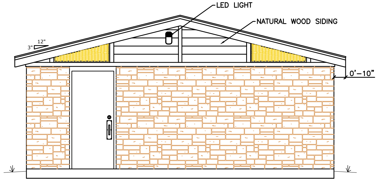
① REAR ELEVATION
