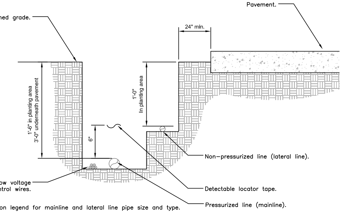
12 IRRIGATION TRENCHING 1 1/2" = 1'-0" FX-IR-FX-AUXEQ-08
