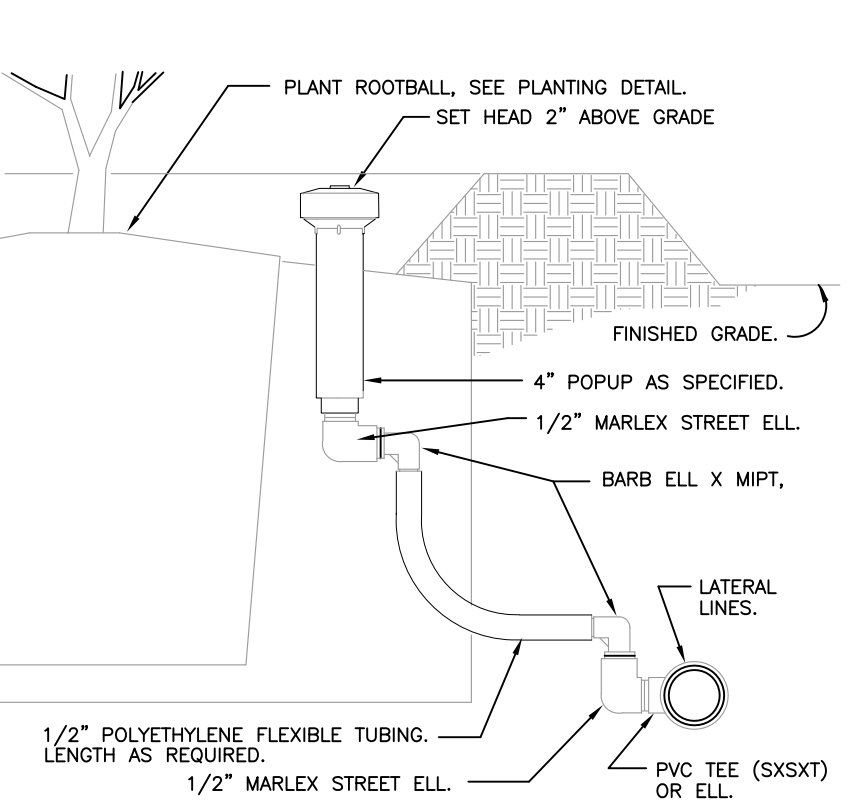
6 POPUP BUBBLER 3" = 1'-0" 32 8403.53-04
