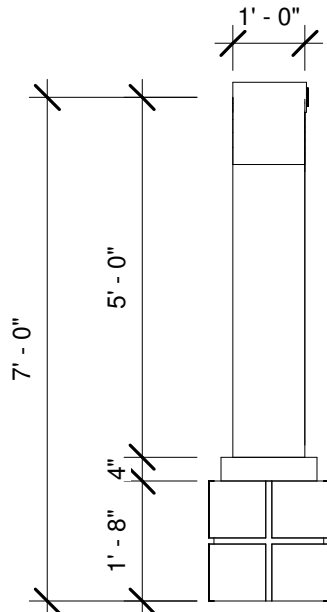
3 SIDE SIGN ELEVATION 3/8" = 1'-0"
