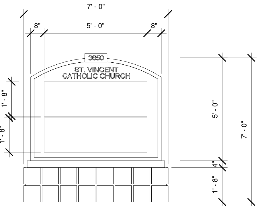
2 FRONT SIGN ELEVATION 3/8" = 1'-0"
