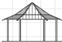
24' MULTI-PITCH HEXAGON SHELTER
