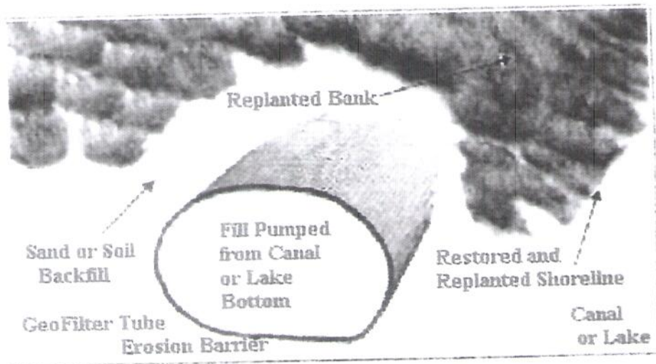
Restoration & Protection of Eroding Lake or Canal Shorelines
