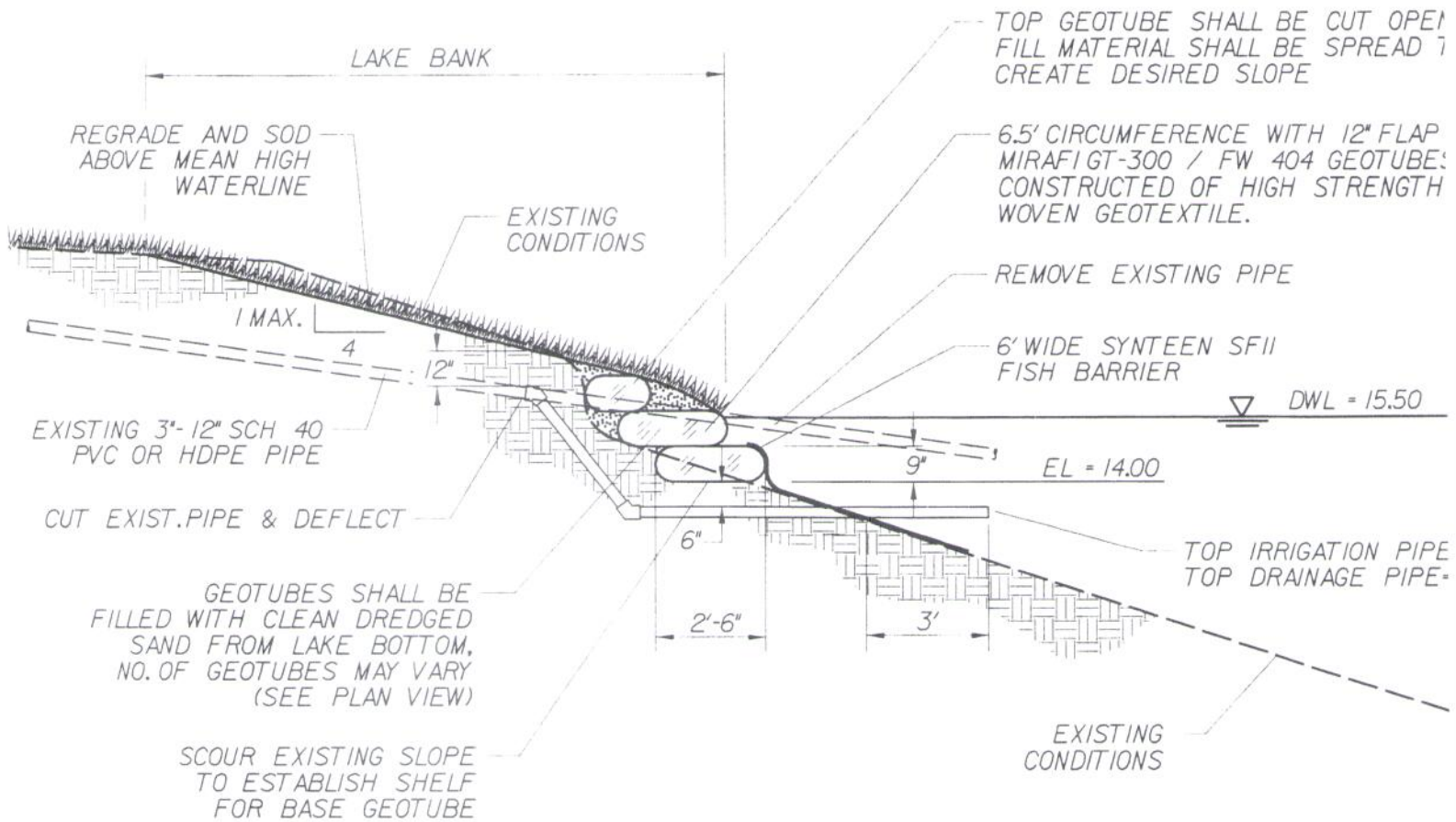
LAKE BANK STABILIZATION DETAIL (GEOTUBE INSTALLATION) NOT TO SCALE
